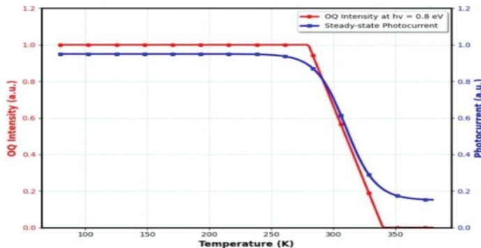
Figure 2. Temperature dependence of (a) optical-quenching intensity at h\nu = 0.8 eV and (b) steady-state photoconductivity I_0 for CdS:Rb . The red curve (circles) shows the OQ intensity remaining approximately constant up to about 280 K, then decreasing progressively and
