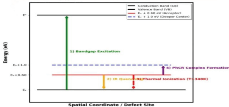
Figure 3. Proposed energy-level diagram and recombination mechanism for Rb-doped CdS and CdS_{1-x}Se_x single crystals. The diagram illustrates the two deep acceptor-related levels at approximately E_v + 0.60 \text{ eV} (red solid line) and E_v + 1.0 \text{ eV} (blue dashed line). The green arrow indicates bandgap excitation, the orange arrow indicates IR-induced quenching, the red dashed arrow indicates thermal ionization above 340 \text{ K} , and the purple arrow indicates photoinduced complex formation after PhCR.
