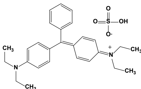
Fig. 1: The chemical structure of Brilliant Green dye.
